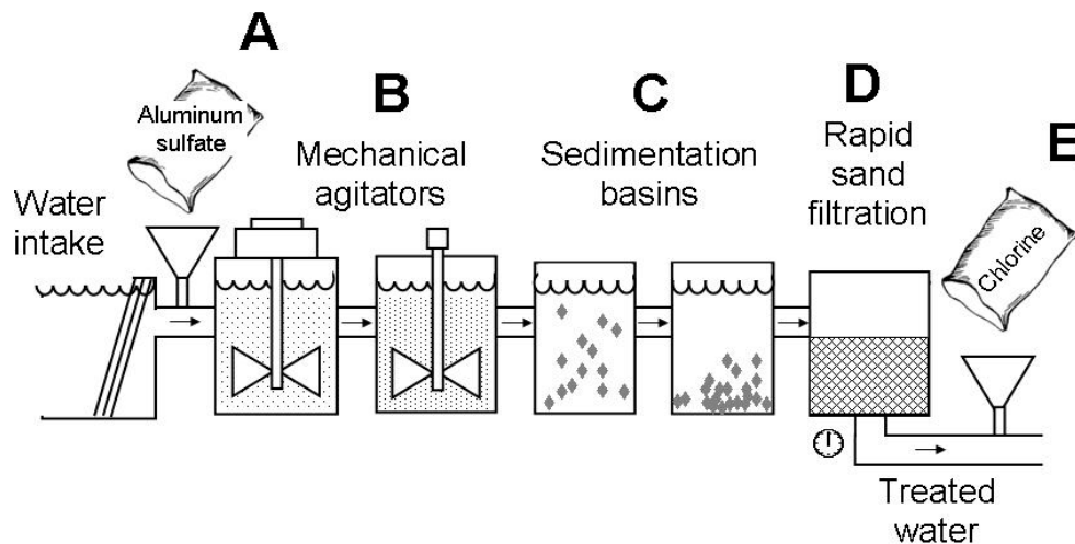
Figure 3. Diagram of Carrollton water treatment process.
